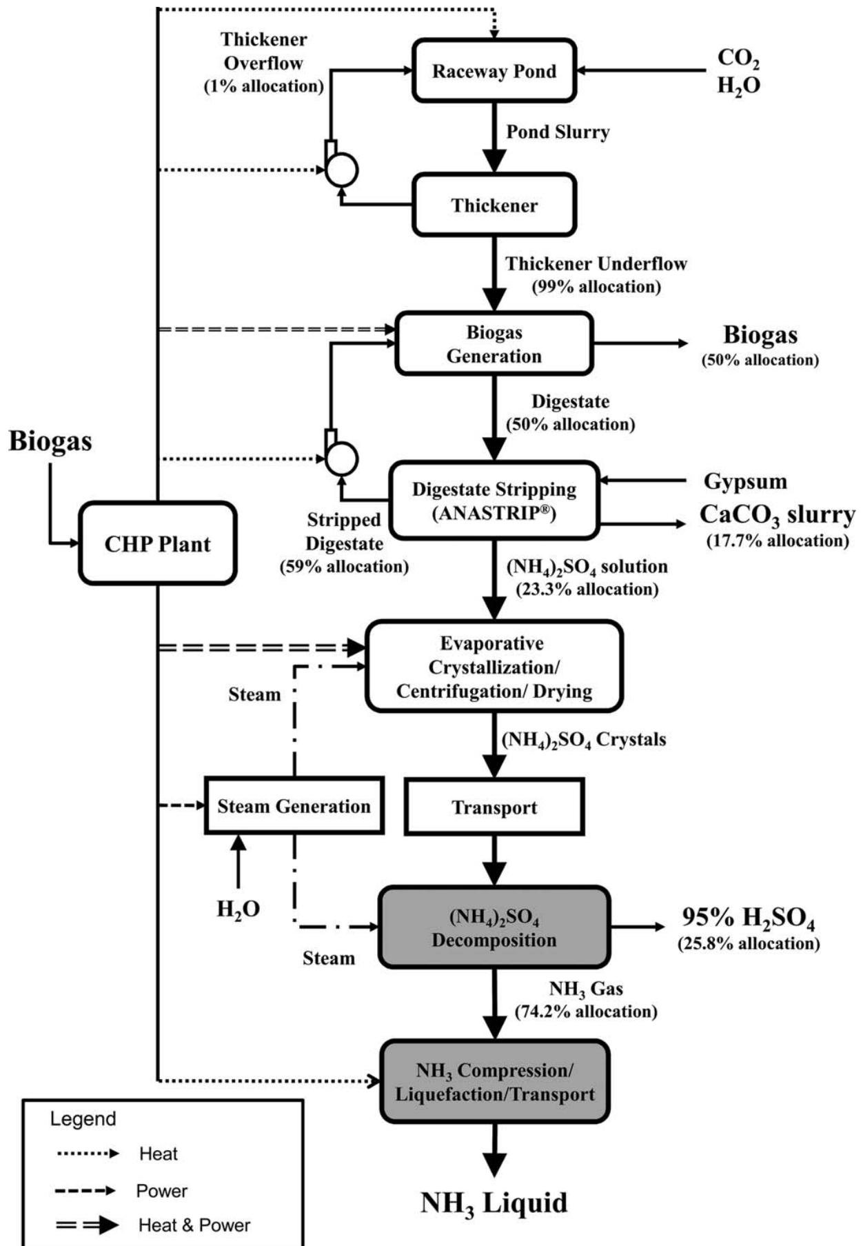
Figure 1. Flow diagram of proposed process. Shaded boxes are new processes added to those reported in Razon [15].
